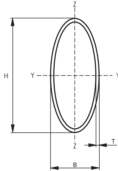
Figure B.4 — Elliptical hollow section
